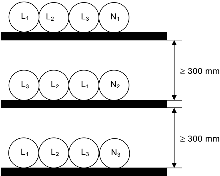
Figure H.52.5 – Special configuration for 9 parallel single-core cables above each other (see 523.7)
